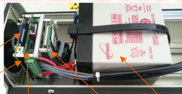
Memory Card Camera Board Power Management, Solar Regulator, Light Control & Wireless Receiver Module 3G Cellular Modem Sealed Lead Acid (SLA) Battery
